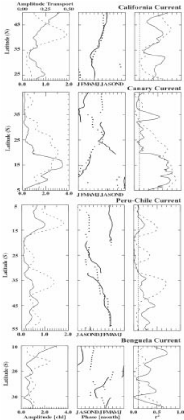
Figure 3. Amplitudes and phases of the seasonal maximum and an estimate of the variance explained ( r^2 , showing 95% confidence level) for a least squares fit annual plus semi-annual harmonic at each latitude to the 3 years of SeaWiFS chlorophyll ( \text{mg m}^{-3} , solid line) and the co-incident 3 years of cross-shelf Ekman transport ( \text{m}^3\text{m}^{-1}\text{s}^{-1} , broken line). Phase is plotted with summer centered in each hemisphere.
